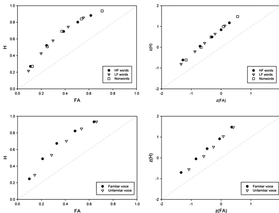
Fig. 1. Group-level receiver operating characteristic (ROC, left panel) and z-ROC (right panel) plots. The upper plots present data by word type, and the lower plots present data by voice status (familiar versus unfamiliar).
